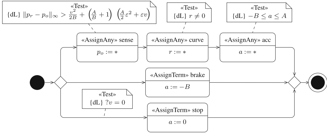
Fig. 10 The controller of the robotic obstacle avoidance model
