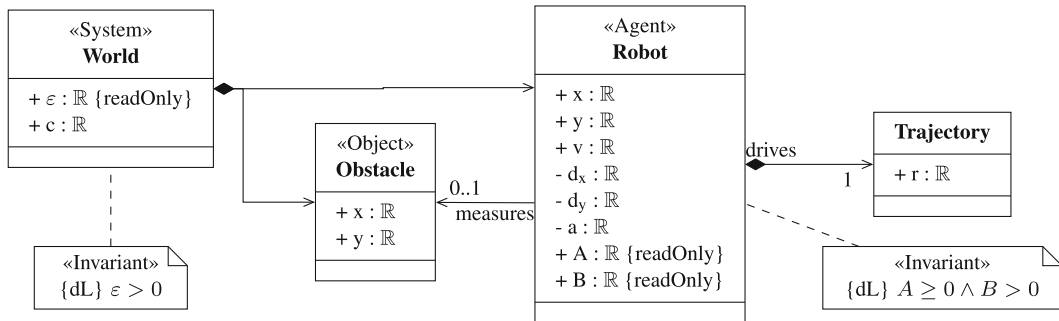
Fig. 8 The structure of the robotic obstacle avoidance model
