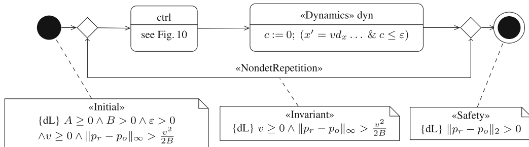
Fig. 9 Overview of the behavior of the robotic obstacle avoidance model. The model is structured hierarchically, with details on ctrl specified in Fig. 10
