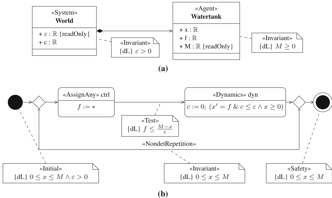
Fig. 2 Example of a hybrid system: a water tank. a The structure of the water tank model: the current water level x must not exceed the maximum level M when the flow f is chosen once every \varepsilon time units, which will be triggered by the clock c . b The behavior of the water tank model: the controller ctrl chooses a new nondeterministic value for the flow f , such that it satisfies the subsequent test before it is passed to the continuous dynamics dyn . Controller and continuous dynamics are repeated nondeterministically many times (which means it can be skipped entirely, cf. Table 1 and the hybrid program UML semantics in Table 2)
