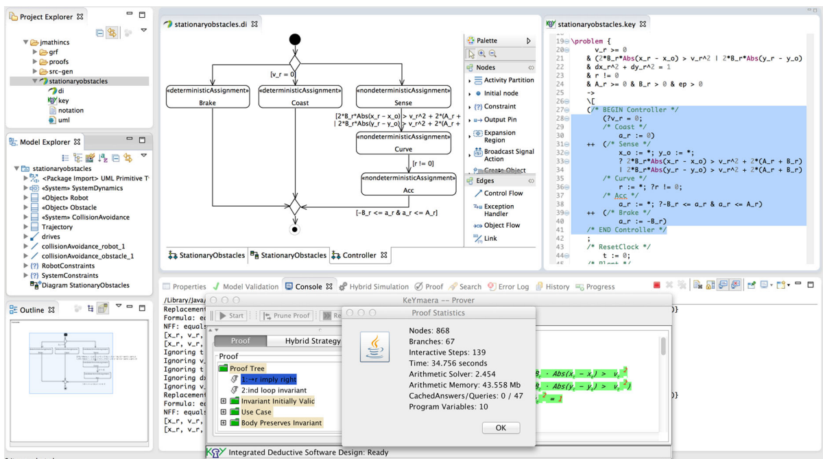
Fig. 4 Screenshot of the textual and graphical modeling editors and a proof in KeYmaera (details on the textual and graphical syntax are described in Sect. 3.5). The left-most three panels , from top to bottom , show the project explorer of Eclipse (access to models and proofs), a hierarchical tree view of the graphical model, and a miniature outline of the graphical model. The graphical editor is displayed in the center of the tool with the textual editor to the right . The text editor selection highlights the controller part that is displayed in the graphical editor. The bottom-most panel shows the KeYmaera theorem prover with its console output in the background
