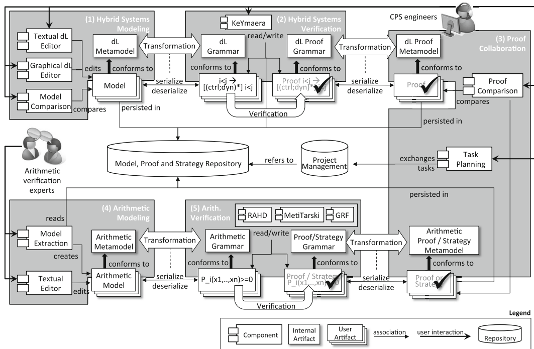
Fig. 1 Overview of components in the verification-driven engineering toolset. The toolset provides components for (1) hybrid systems modeling, (2) hybrid systems verification, (3) proof collaboration, (4) arithmetic modeling, and it provides or uses off-the-shelf components for (5) arithmetic verification. It uses further off-the-shelf components as repositories in the backend
