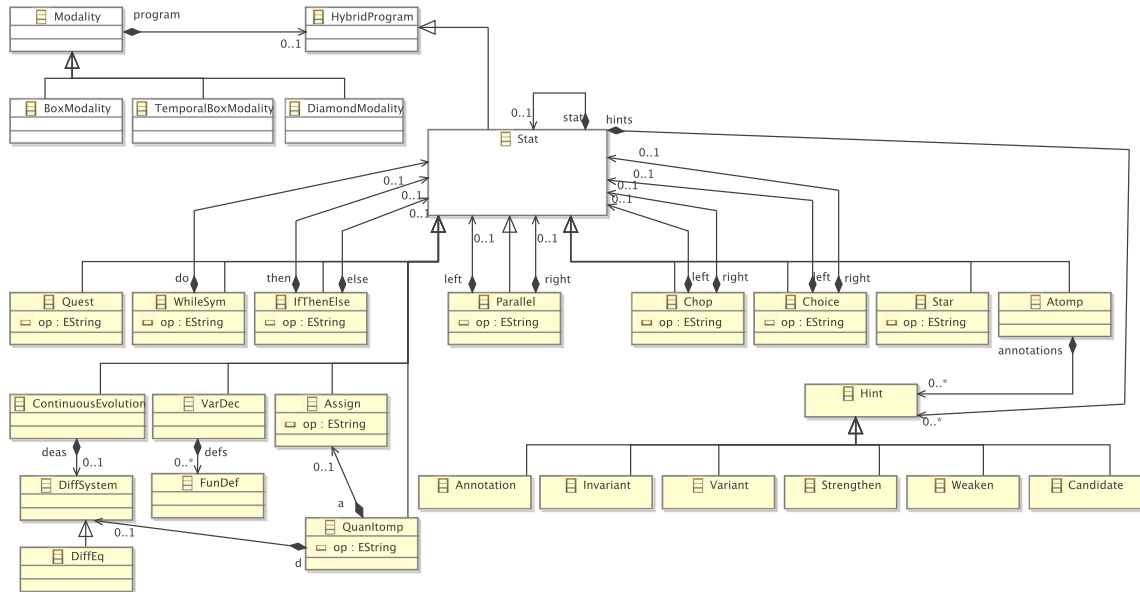
Fig. 3 The d\mathcal{L} metamodel extracted from the input grammar of KeYmaera
