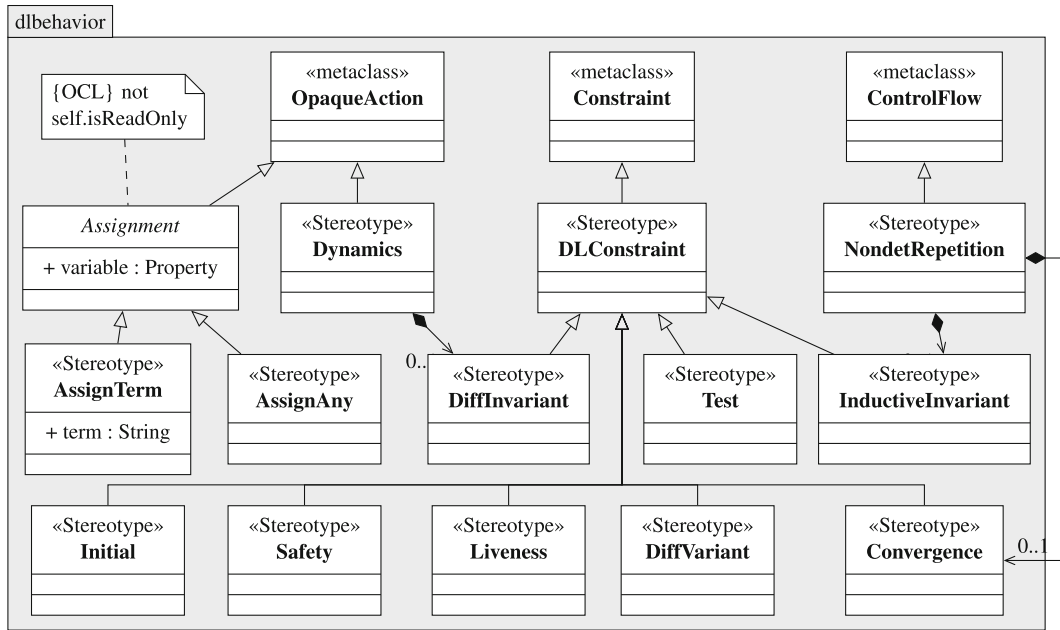
Fig. 6 The Hybrid Program UML profile: behavior of hybrid programs
