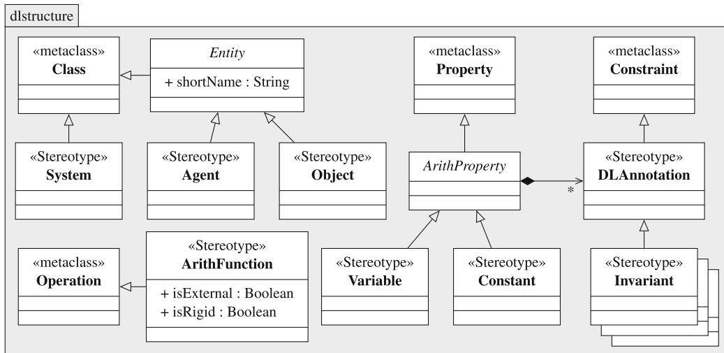
Fig. 5 The Hybrid Program UML profile: structure of hybrid programs
