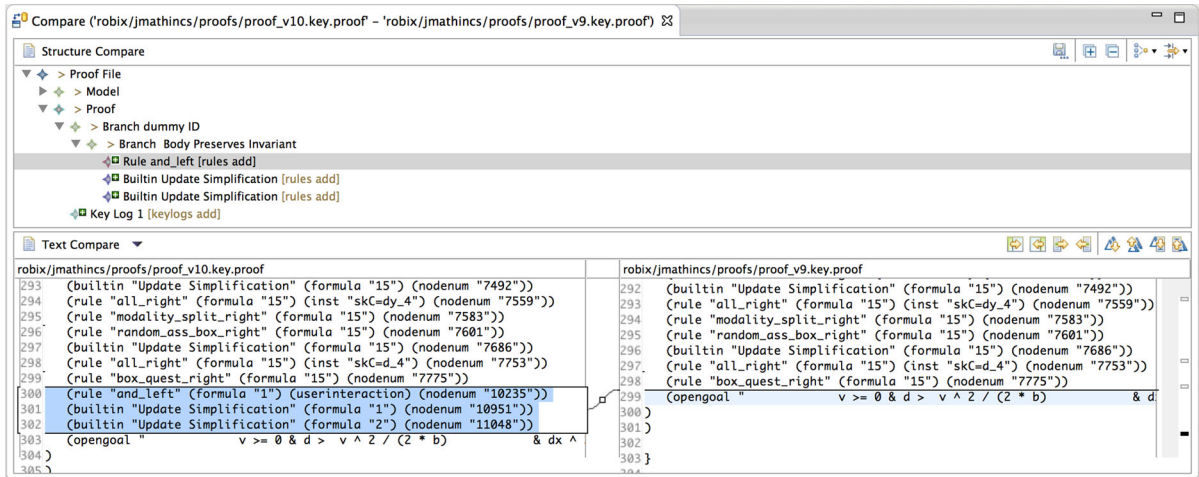
Fig. 7 Comparison of the structure of two proof versions
