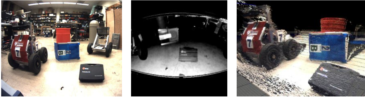
(a) raw camera image (b) LIDAR depth and intensity (c) resulting colored 3D point cloud
